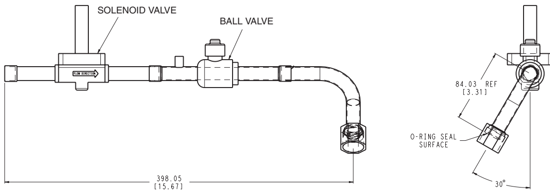
TUBE ASSEMBLY 00PSN500175200A
